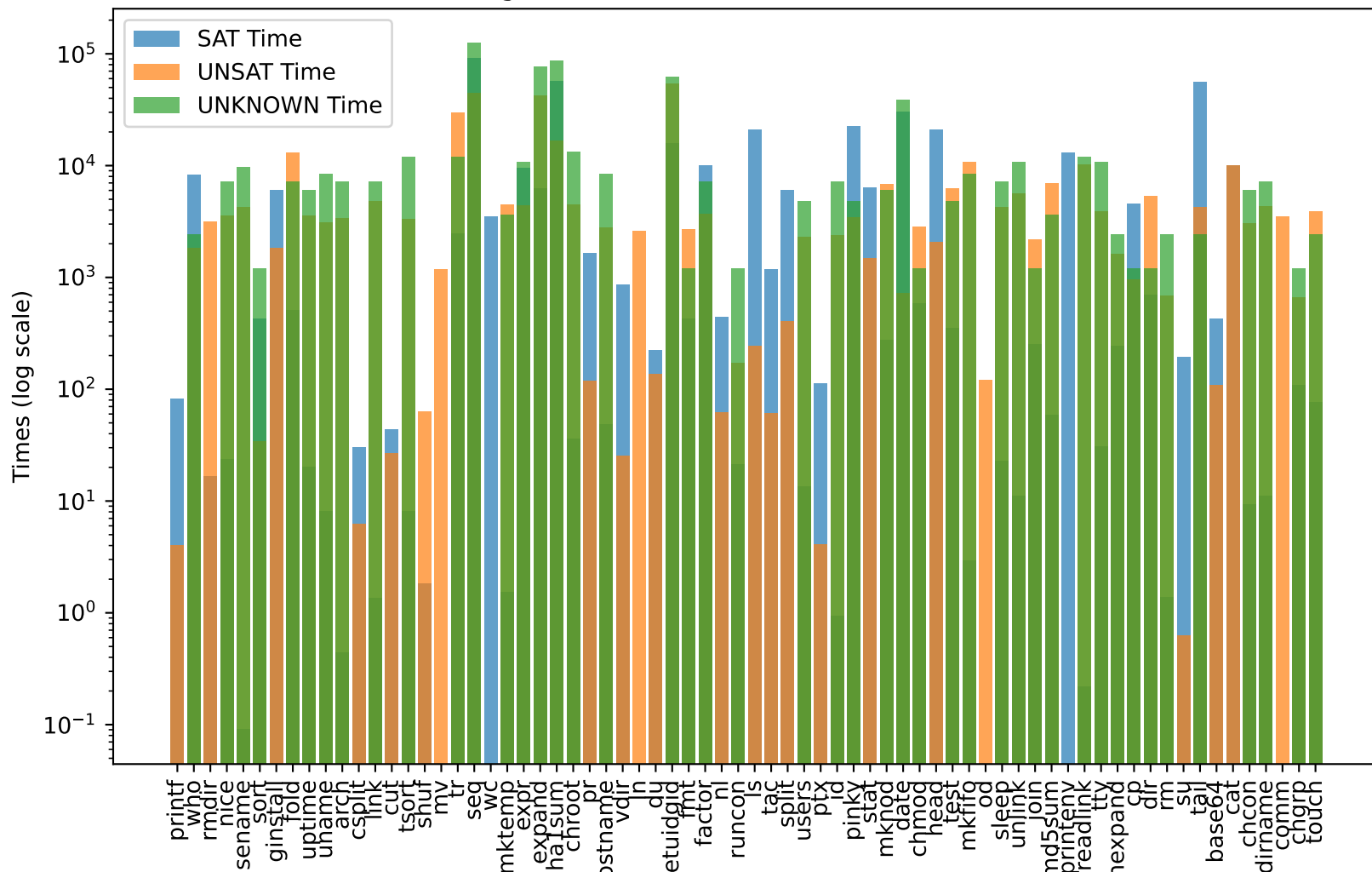
gnu - SAT, UNSAT, UNKNOWN Times
